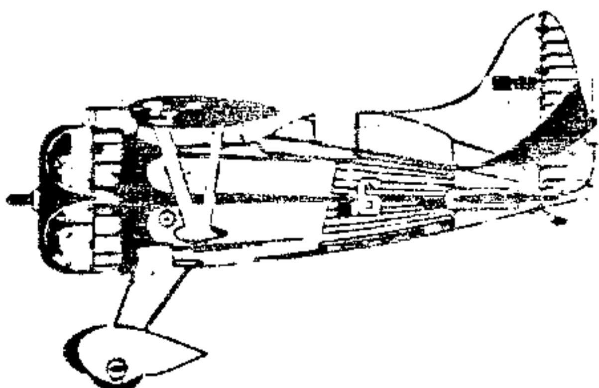
RC "Quick Links" make ideal attachment fittings for wing struts, suggests Tom Wenzel, Plainview, N. Y. Plywood mounts built into wing for easy attachment. Struts pop free in event of a crash.
