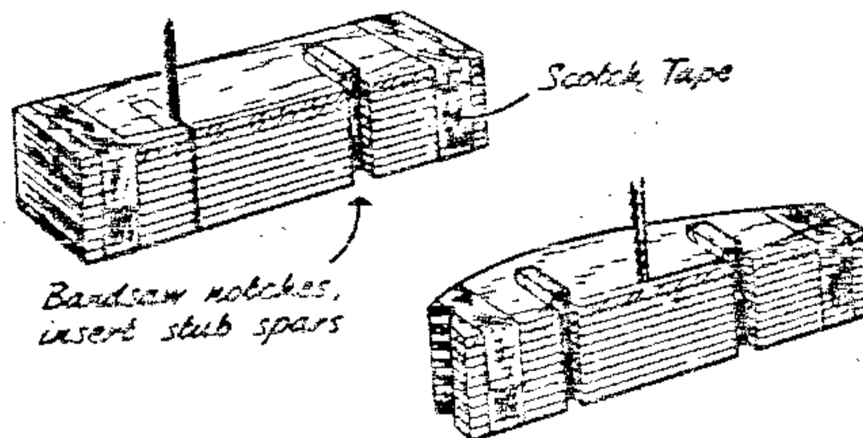
● Here's another rib-cutting scheme, this one from Don Nelson, Portland, Ore. Scotch Tape holds stack of sheets till spar slots are sawed; tight fitting stub spars hold for outline sawing.
